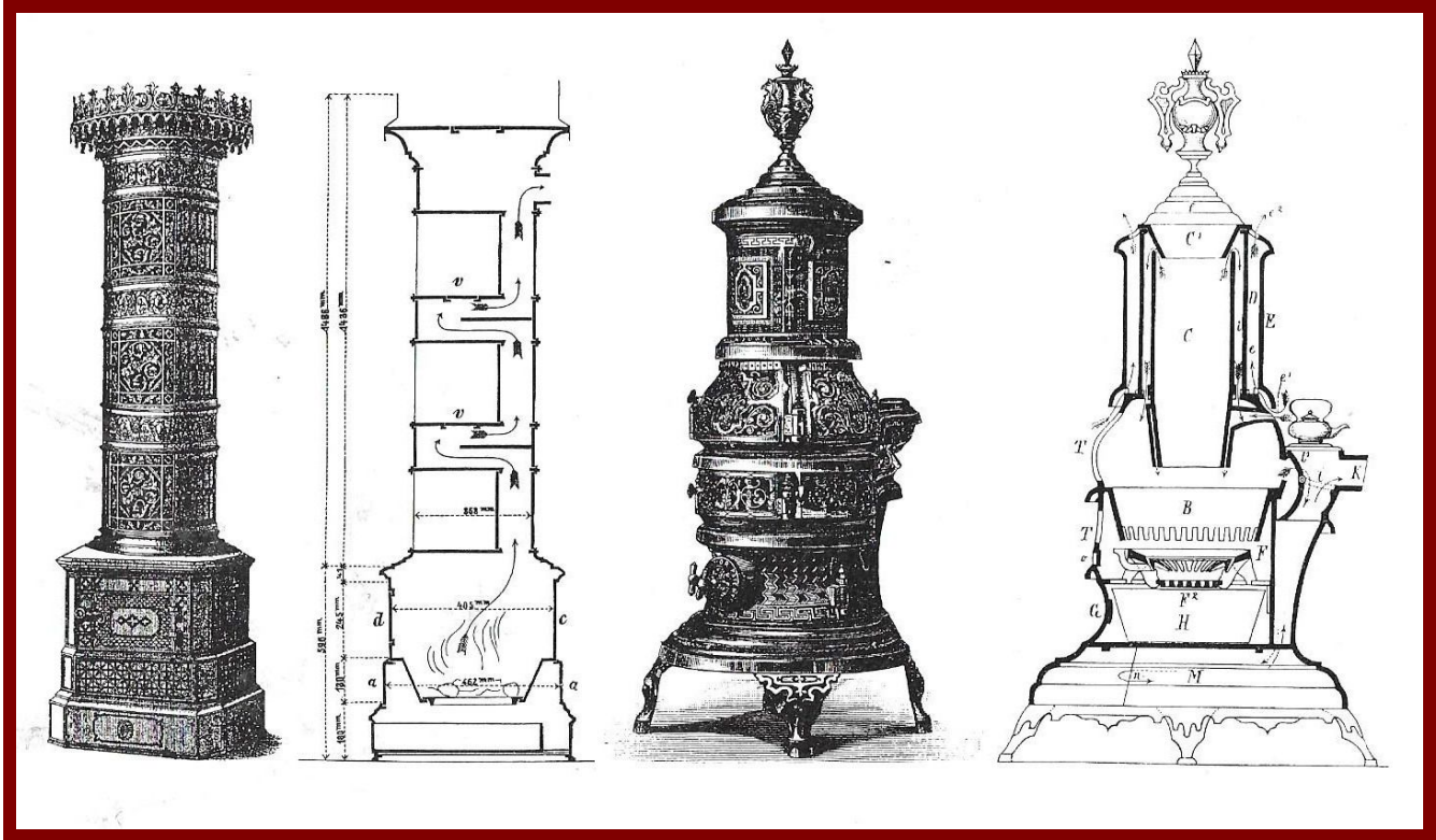
A selection of Swiss stoves from 1867 (Sulzer)
